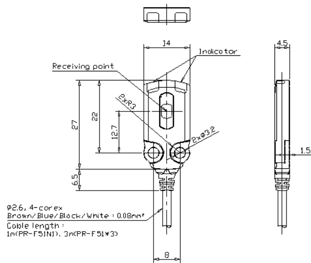
Receiver
